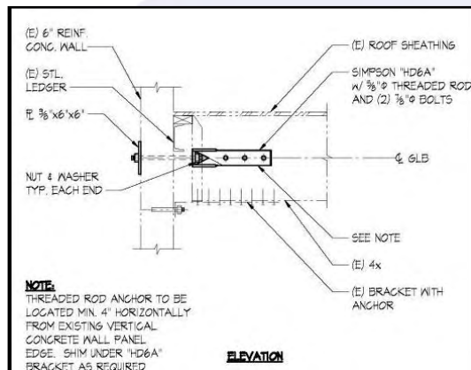
Example roof-to-wall anchorage retrofit of tilt-up structure
